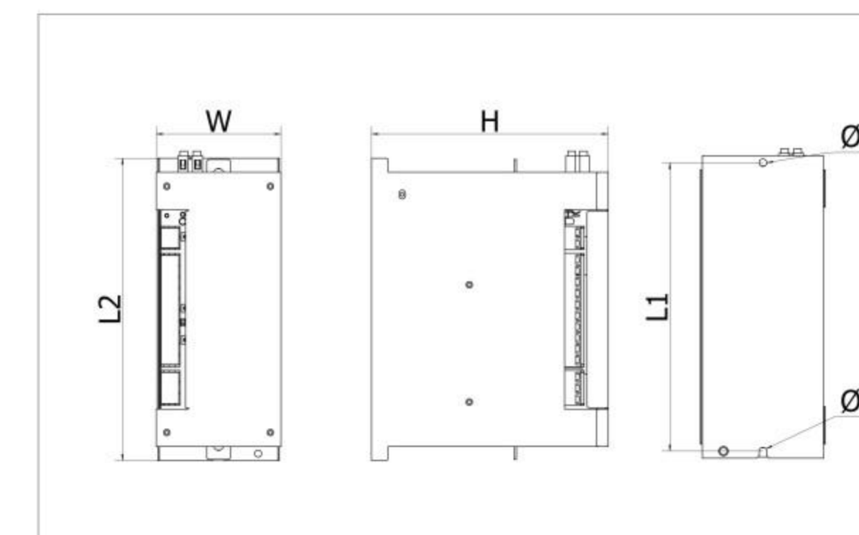
图十 (RK16P-外型及安装图)
