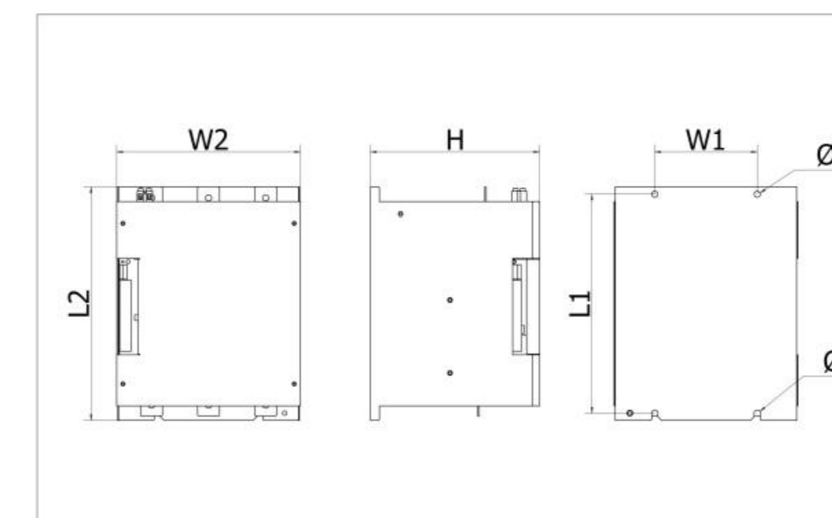
图八 (RKZ3-外型及安装图)
