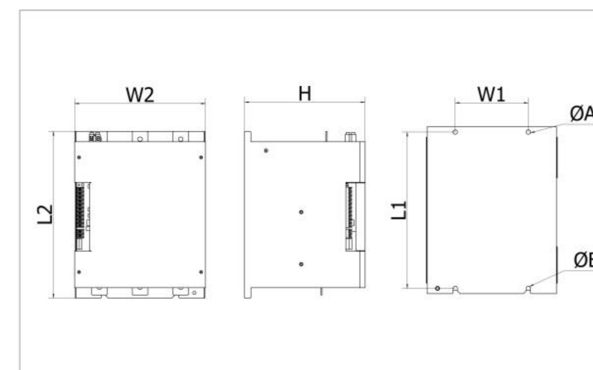
图七 (RK33P-外型及安装图)
